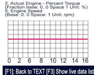
Chart Mode
