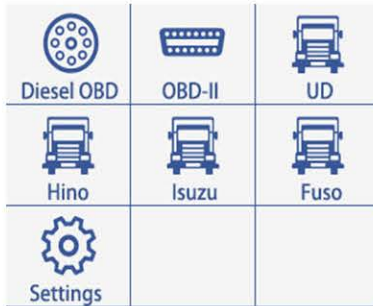
Home Menu
