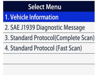
Scan Options
