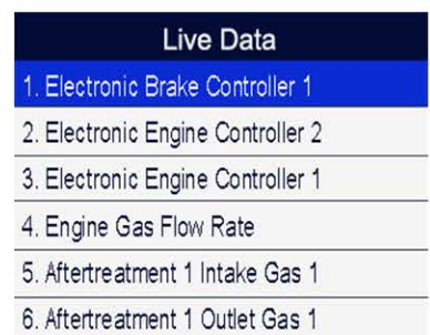
Sensors data
