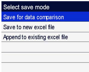
Data Export
