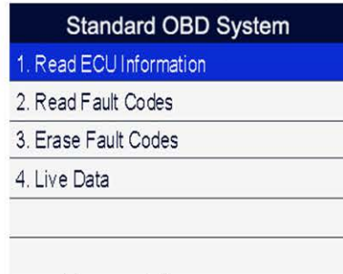
Home Menu
