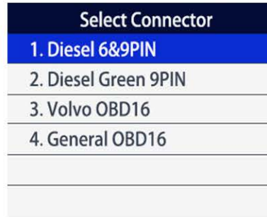
Connector Options
