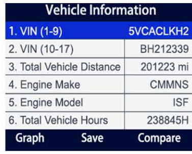
Vehicle Info
